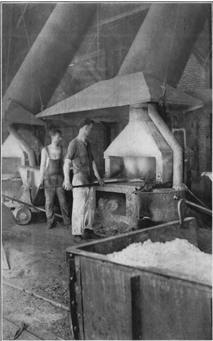
PLATE 2.—ORE HEARTH OR SCOTCH HEARTH.
