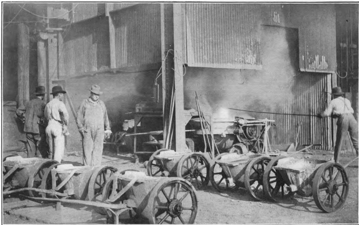
PLATE 7.—BLAST FURNACE DURING SLAG TAPPING.
