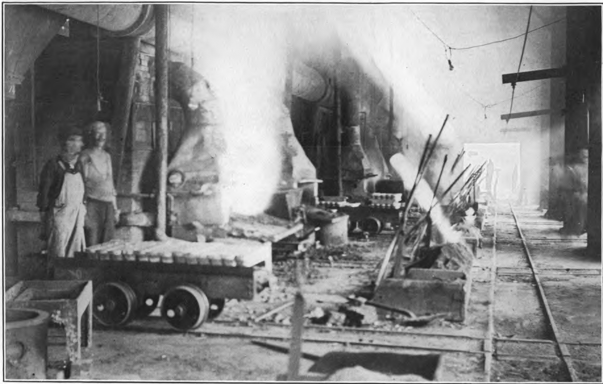
PLATE 3.—ORE HEARTH BUILDING IN PARTIAL OPERATION.
