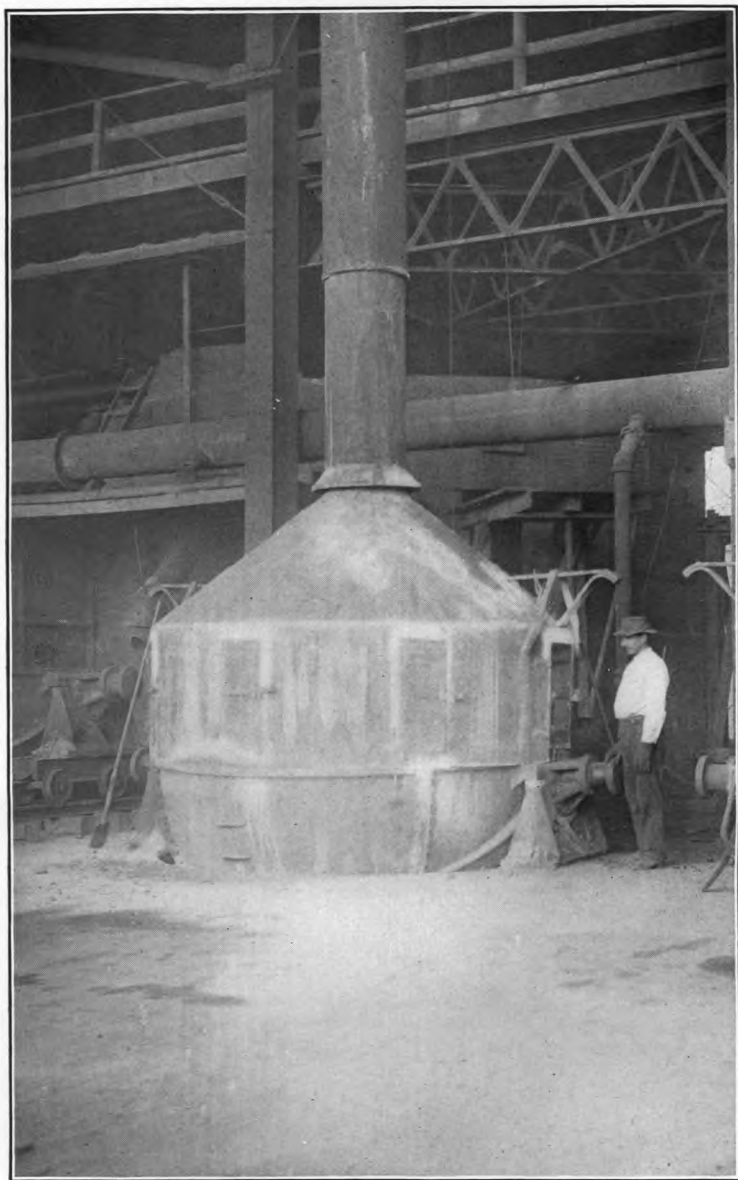
PLATE 4.—HUNTINGTON-HEBERLEIN POT.
